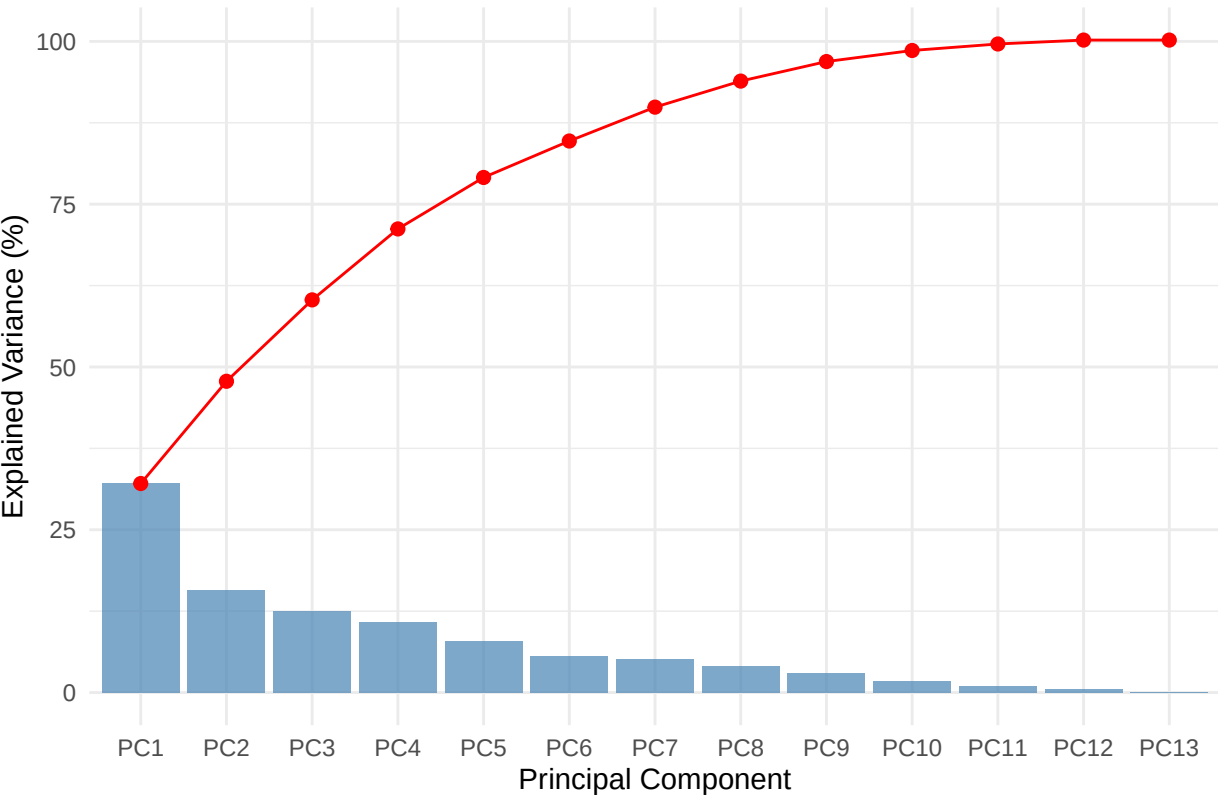
Explained and Cumulative Variance by PC
